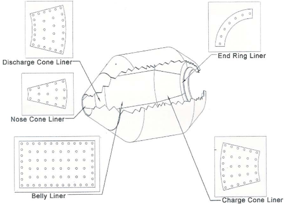
Mixer Drum Poly Liner Break Out Diagram
