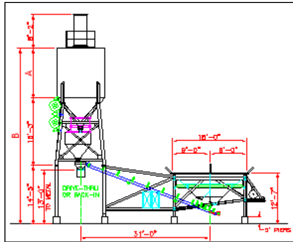
DC Colt Decumulating Plant Typical Layout
